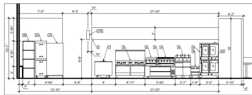
FOOD SERVICE ELEVATION 1
