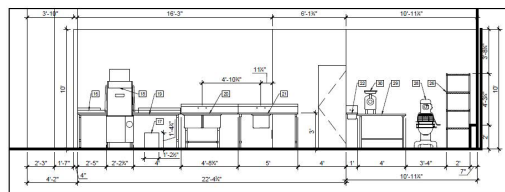
FOOD SERVICE ELEVATION 2
